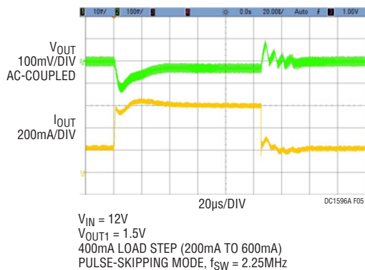
Figure 5. Load Step Response
