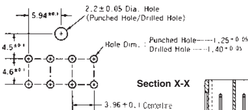
PC Board Layout (Applicable Board Thickness: 1.6 mm)
