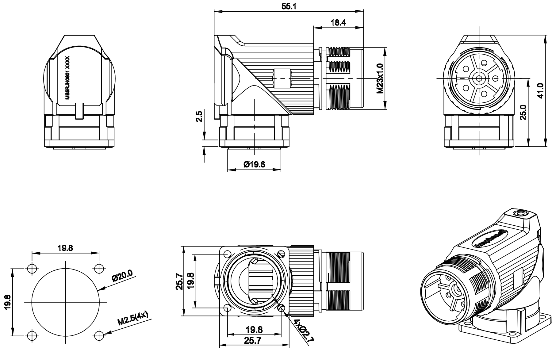
MOUNTING HOLE
