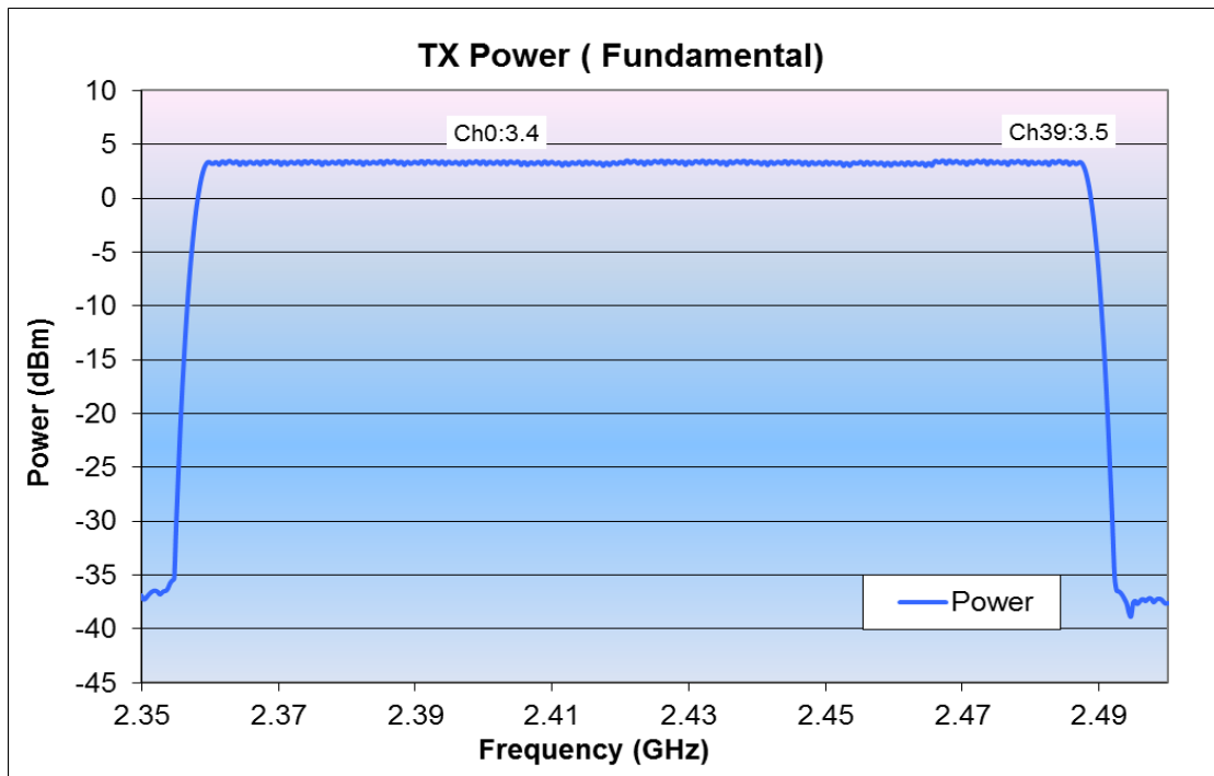
Figure 7. TX power
