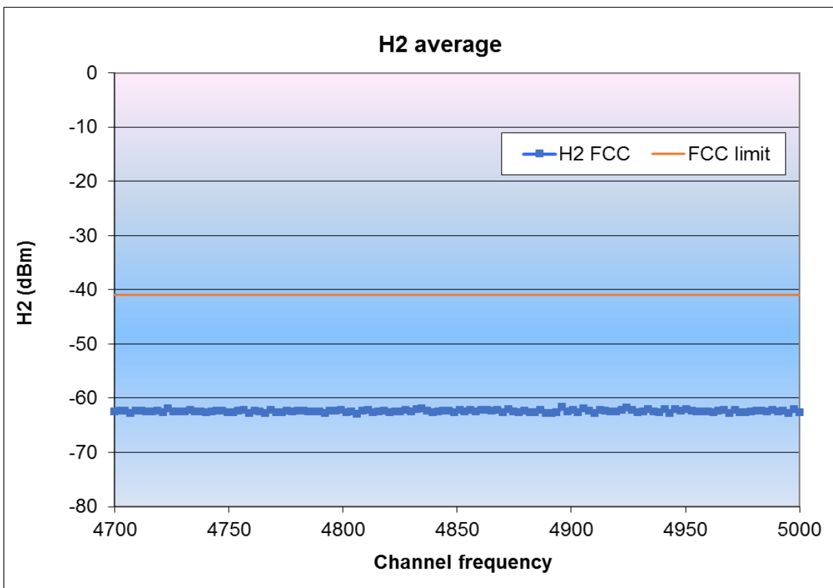
Figure 17. Conducted H2 FCC spurious
