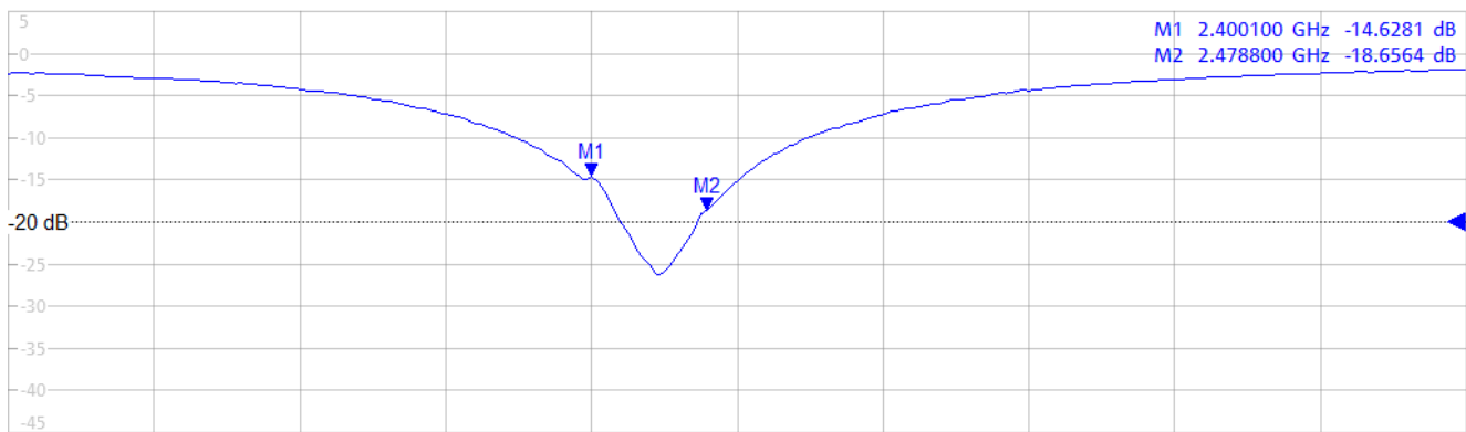
Figure 56. S11 diagram (Rx mode)
