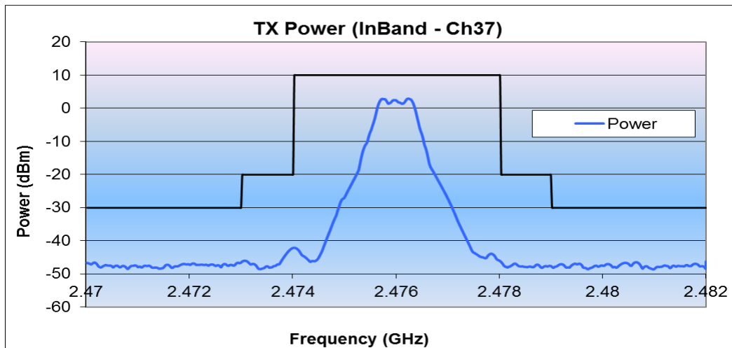
Figure 11. TX power in band (channel 37)
