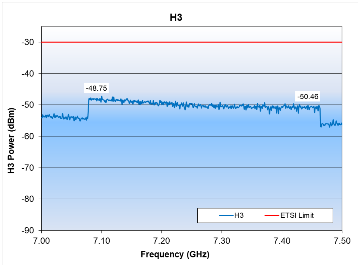
Figure 23. Conducted H3 spurious
