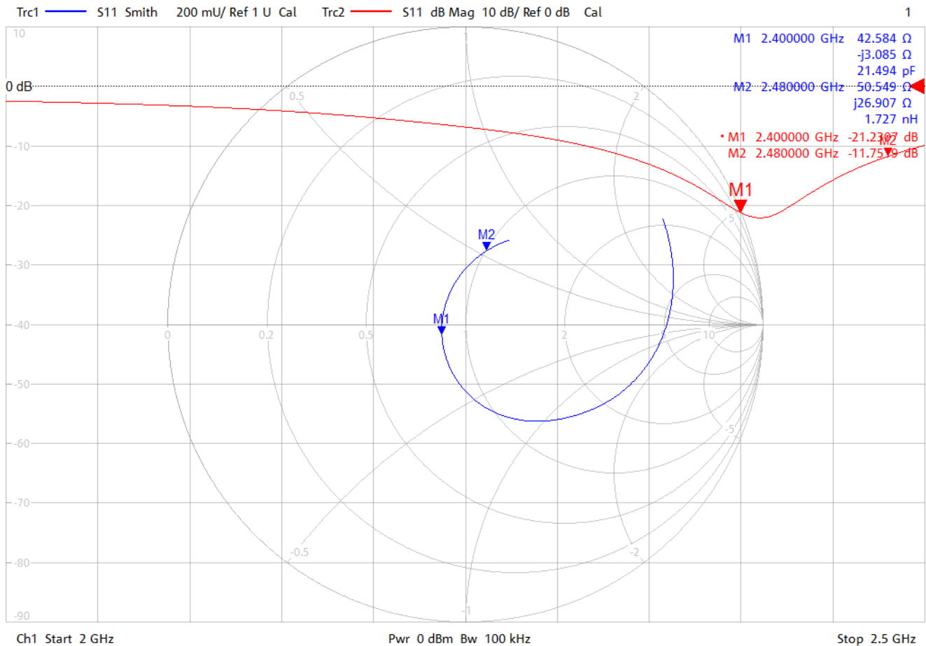
Figure 54. S11 diagram (Rx mode)
