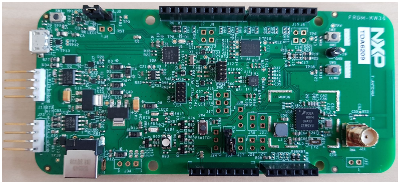
Figure 2. Freedom development kit for Kinetis/FRDM-KW36Z
