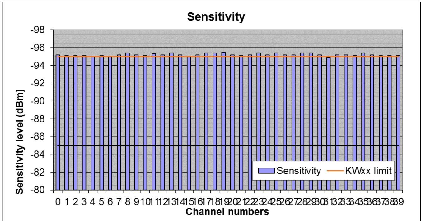
Figure 46. Sensitivity result
