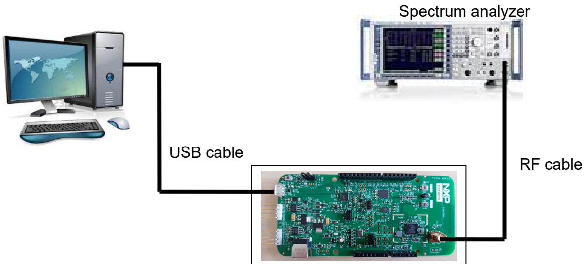
Figure 3. Conducted TX test setup
