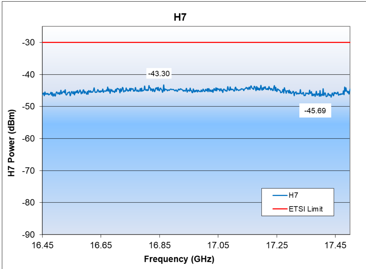
Figure 27. Conducted H7 spurious
