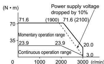
R88M-K5K020F/C (5 kW)
