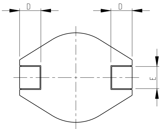
RECOMMENDED LAND PATTERN FOR 3630D & 3630F
