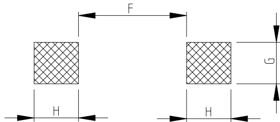
RECOMMENDED LAND PATTERN FOR 3630D & 3630F
