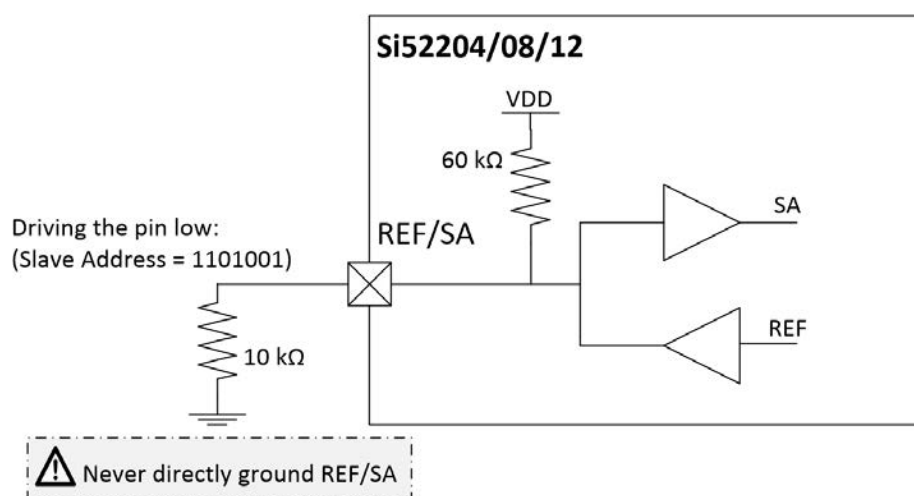
Figure 5.8. REF/SA Pin Function
