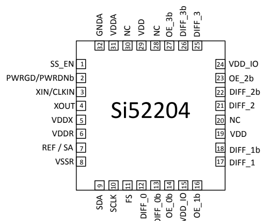
Figure 9.3. 32-pin QFN
