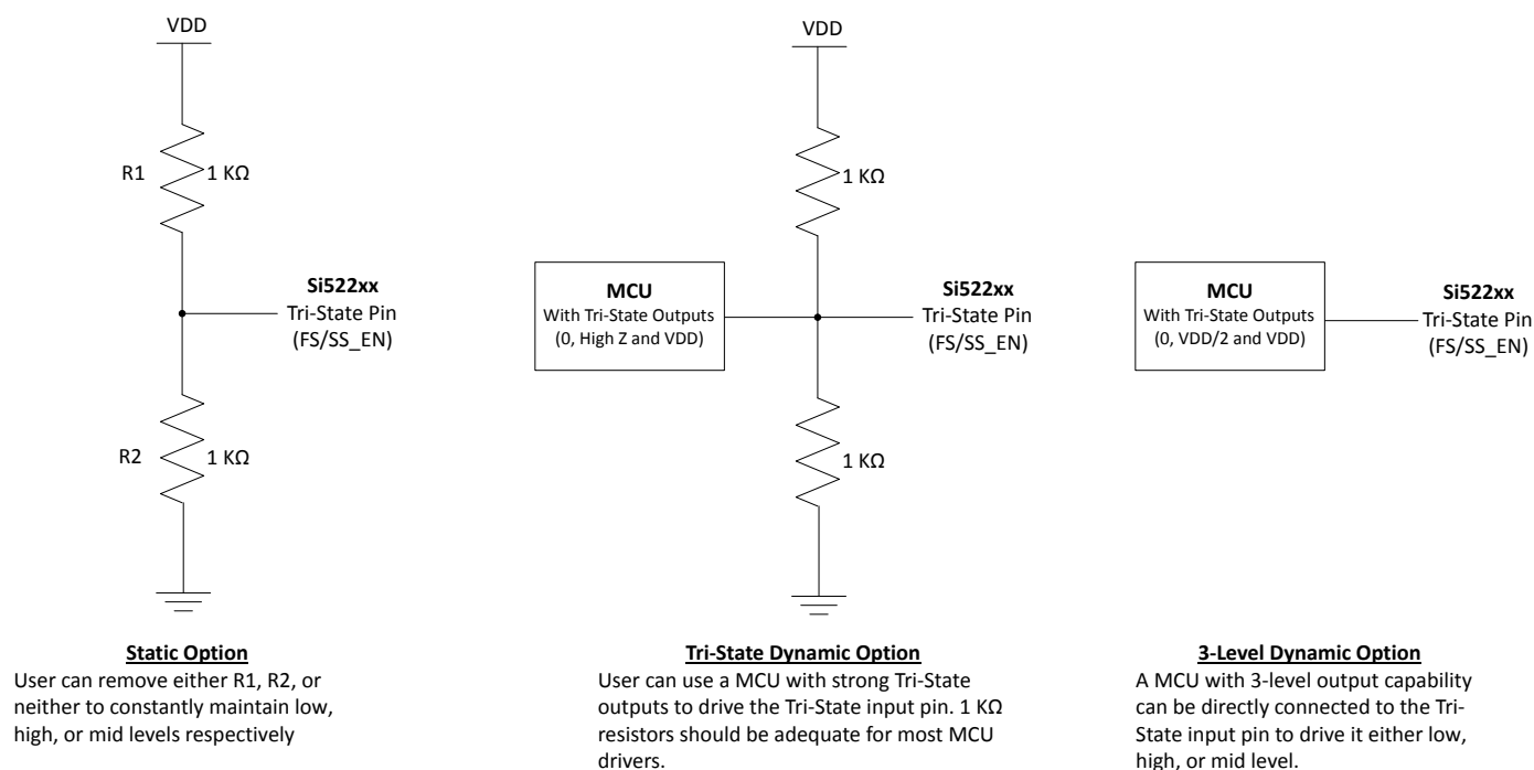
Figure 5.7. Tri-State Pin Schematics
