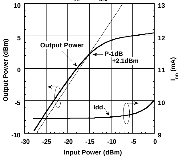
OUTPUT POWER, I_{DD} vs. INPUT POWER ( V_{DD}=3V, V_{cont}=2V, f=938MHz )
