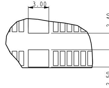
Center smt holddown type
