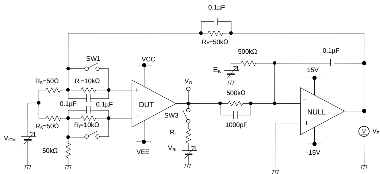
Figure 21. Test Circuit 1
