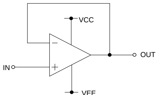
Figure 25. Voltage Follower
