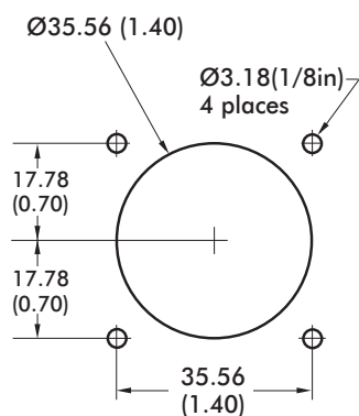
FLUSH MOUNT *
