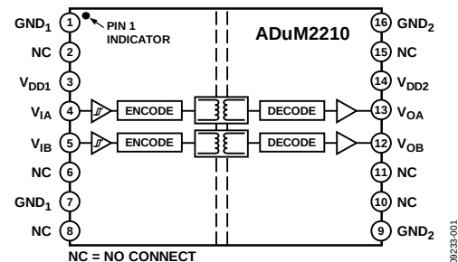
Figure 1. ADuM2210
