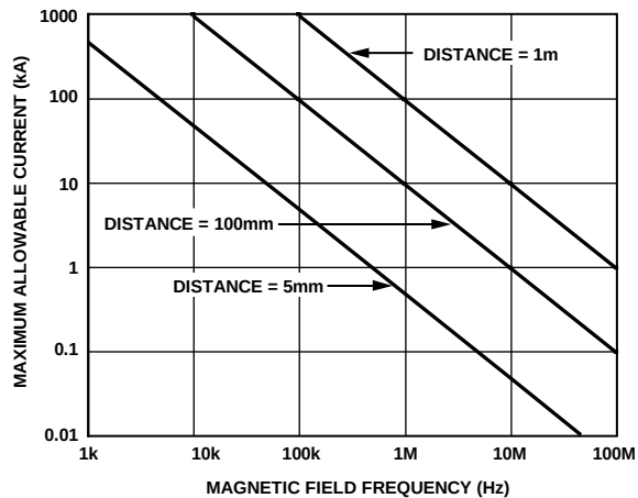
Figure 15. Maximum Allowable Current for Various Current-to-ADuM2210/ADuM2211 Spacings
