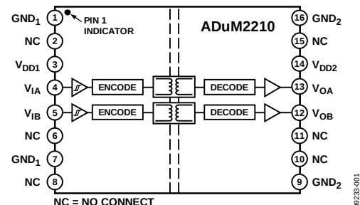
Figure 1. ADuM2210
