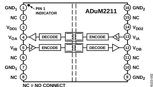
Figure 2. ADuM2211
