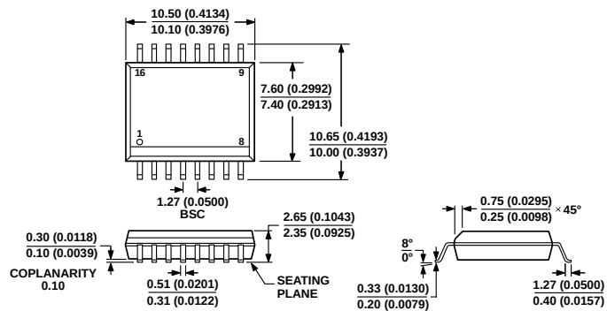
Figure 19. 16-Lead Standard Small Outline Package [SOIC_W] Wide Body (RW-16) Dimensions shown in millimeters and (inches)
