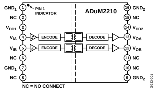
Figure 1. ADuM2210
