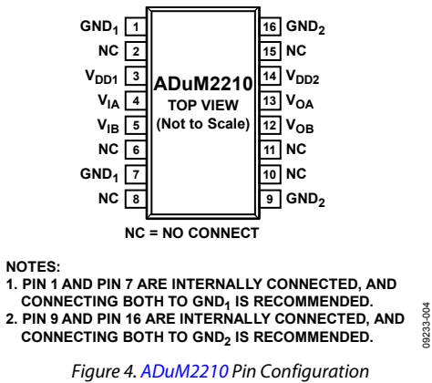
Figure 4. ADuM2210 Pin Configuration
