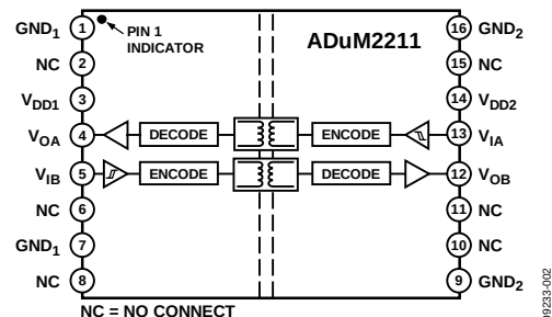
Figure 2. ADuM2211
