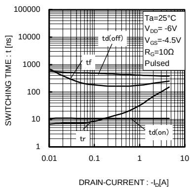
Fig.14 Switching Characteristics
