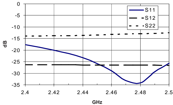
Input/Output Return Loss, Isolation vs. Frequency, T=25^{\circ}C
