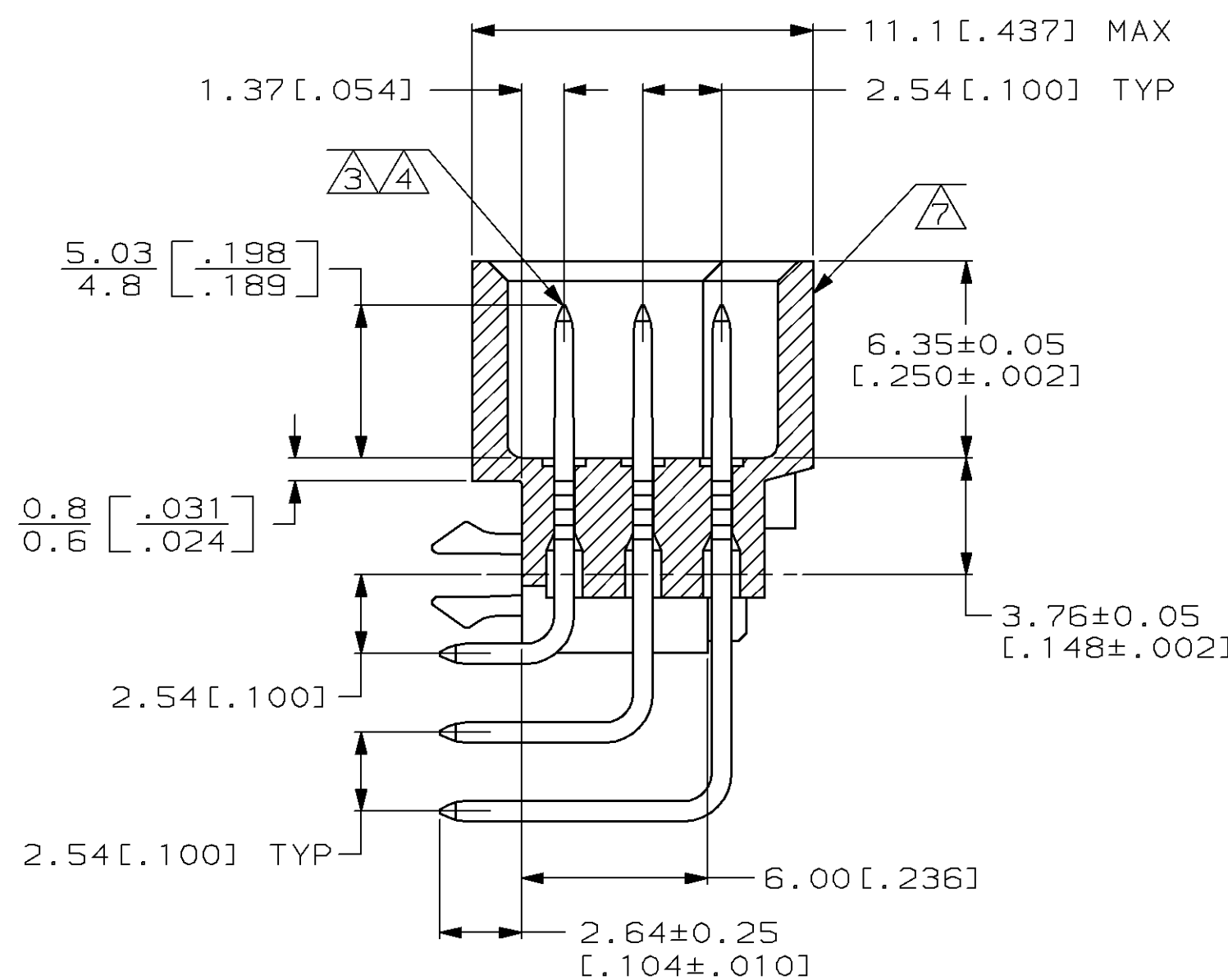
SECTION X-X
