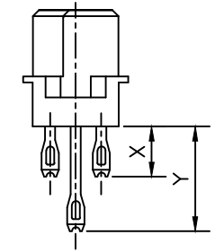
EYELET SHORT/LONG (09/10) MIXED EYELET (08)
