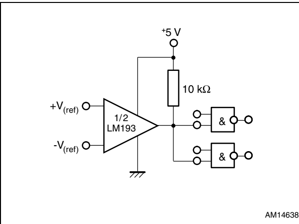
Figure 11. Driving CMOS
