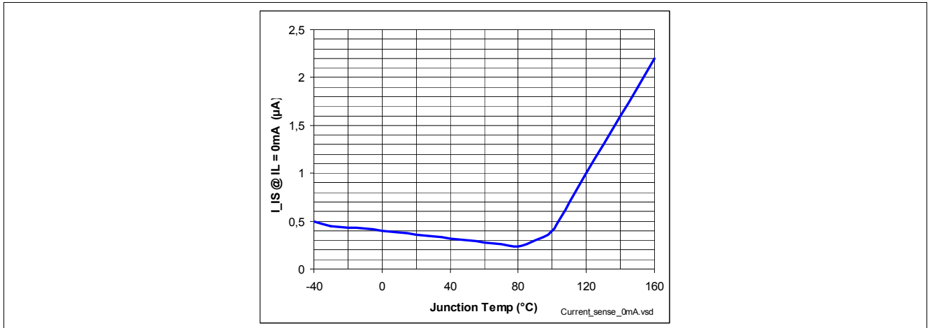
Figure 45 Current Sense at no Load I_S = f(T_J; V_S) , I_L = 0
