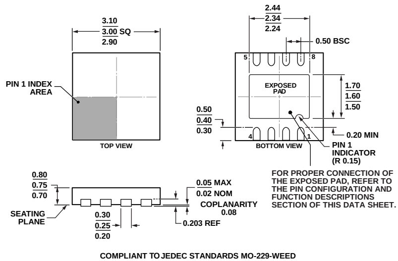
Figure 92. 8-Lead Lead Frame Chip Scale Package [LFCSP_WD] 3 mm × 3 mm Body, Very Very Thin, Dual Lead (CP-8-11)
