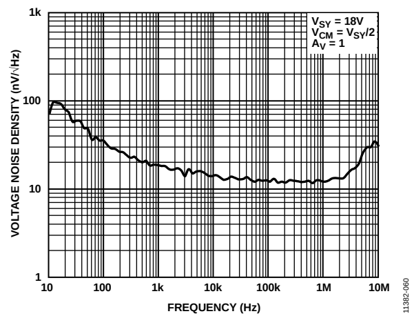
Figure 59. Voltage Noise Density vs. Frequency
