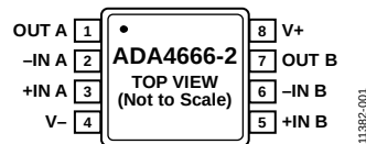
Figure 1. 8-Lead MSOP
