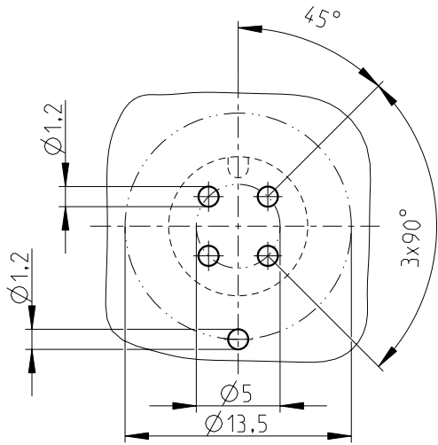
PCB-layout (advice)
