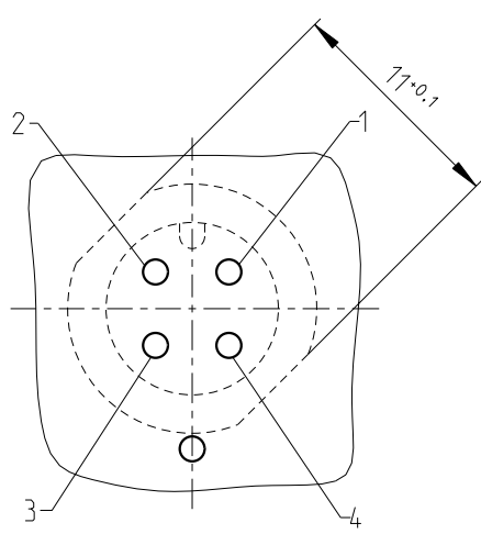
Position PCB-layout to cutout device
