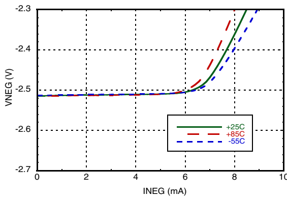
VNEG Load Regulation @ VDD=4V
