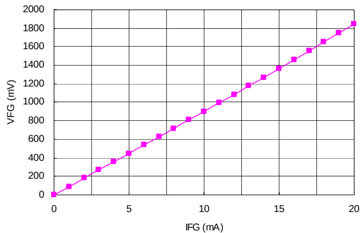
IFG-VFG VDD=5V, IN+=2.5V, IN-=GND MEAS:VFG
