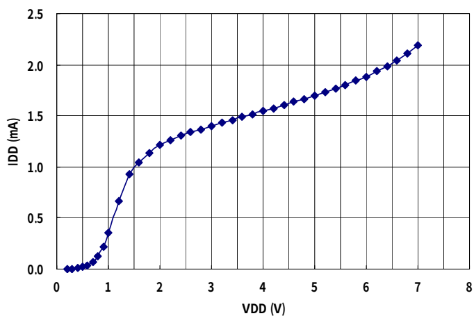
VDD-IDD IN+=VDD, IN-=GND MEAS:IDD
