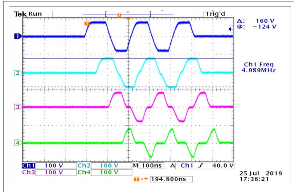
FIGURE 3-15: Sample Waveform from Multiple Channels of the HV7358.
