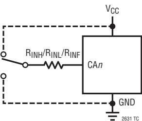
Test Circuit 2
