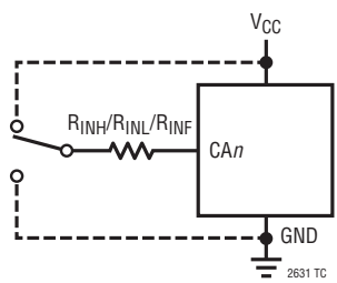
Test Circuit 2
