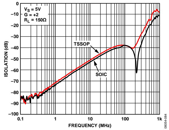
Figure 46. Forward Isolation vs. Frequency (ADA4891-3 Only)
