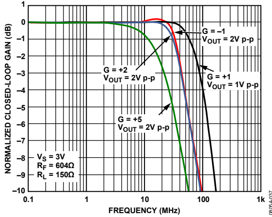
Figure 19. Large-Signal Frequency Response vs. Gain, V_S = 3\text{ V} , ADA4891-1/ADA4891-2
