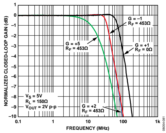
Figure 18. Large-Signal Frequency Response vs. Gain, V_S = 5V , ADA4891-3/ADA4891-4
