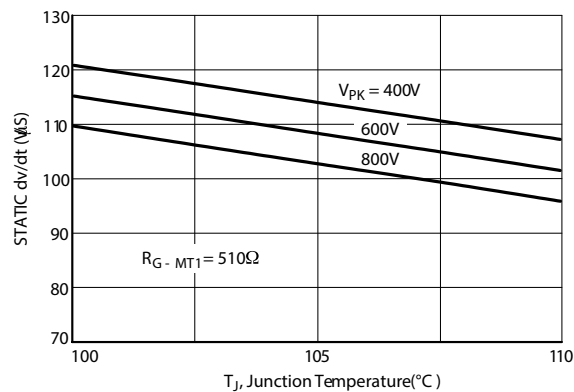
Figure 11. Typical Exponential Static dv/dt Vs. Junction Temperature, MT2(+)
