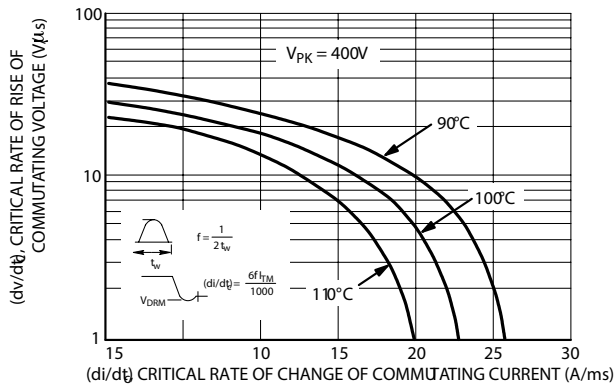
Figure 15. Critical Rate of Rise of Commutating Voltage
