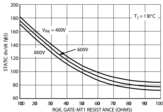
Figure 9. Typical Exponential Static dv/dt Vs. Gate-MT1 Resistance, MT2(+)
