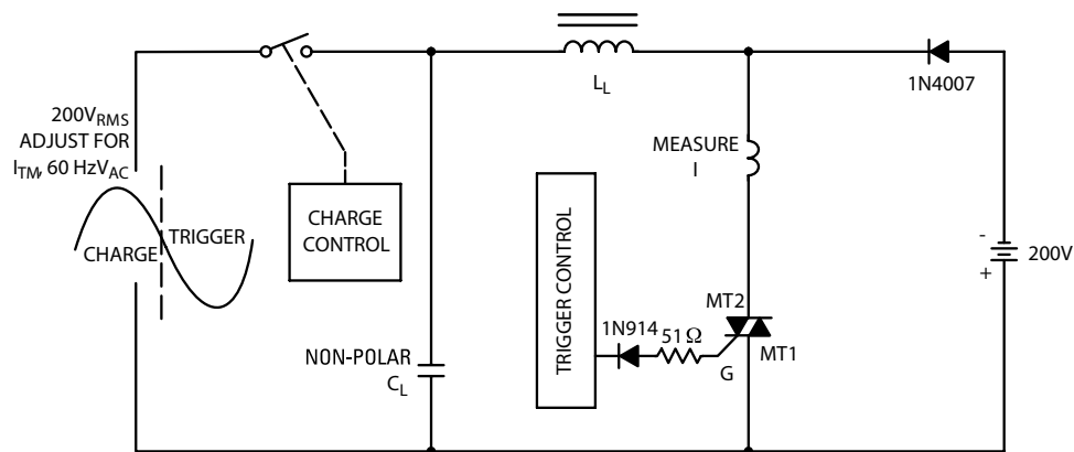
Figure 16. Simplified Test Circuit to Measure the Critical Rate of Rise of Commutating Current (di/dt)
