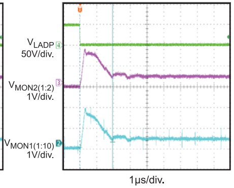
MON1,2 OCP Response - ILIM:2.5mA 0 to 10mA
