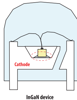
Figure 12: LED Configuration
