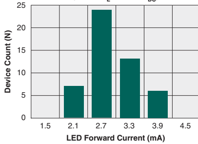
Typical I_F for Switch Operation (N=50, I_L=250mA_{DC} )
