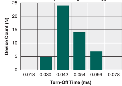
Typical Turn-Off Time (N=50, I_F=5mA , I_L=250mA_{DC} )
