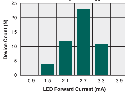
Typical I_F for Switch Dropout (N=50, I_L=250mA_{DC} )
