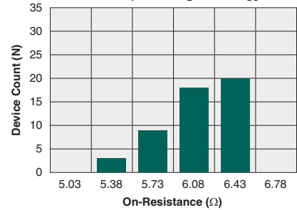
Typical On-Resistance Distribution (N=50, I_F=5mA , I_L=250mA_{DC} )
