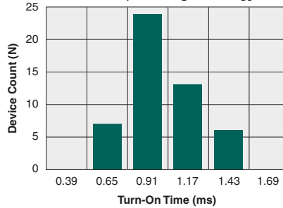
Typical Turn-On Time (N=50, I_F=5mA , I_L=250mA_{DC} )
