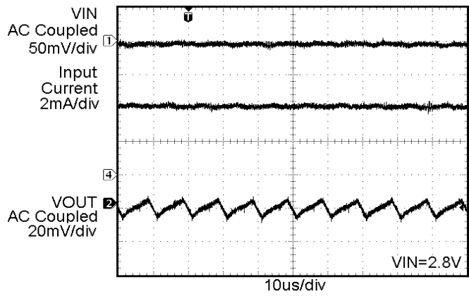
Figure 18. Operating Waveforms in 1.33x Mode
