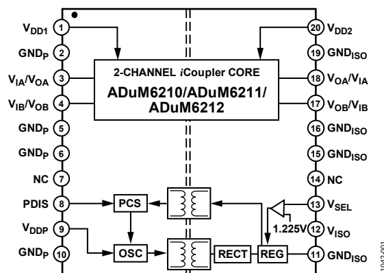
Figure 1. ADuM6210/ADuM6211/ADuM6212
