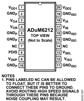
Figure 5. ADuM6212 Pin Configuration
