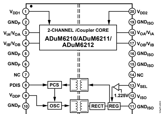
Figure 1. ADuM6210/ADuM6211/ADuM6212
