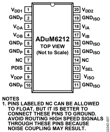
Figure 5. ADuM6212 Pin Configuration
