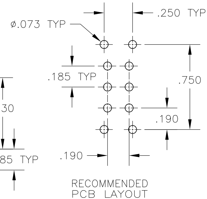
PRINTED CIRCUIT
