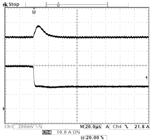
Fig-2.0V-7: Output voltage response for Vout=2.0V to negative load current step change from 30A to 15A with slew rate of -5A/us at Vin=12V. Co=47uFx2 ceramic. Top trace: output voltage (200mV/div.) Bottom trace: load current (10A/div.) Time scale: 20us/div.
