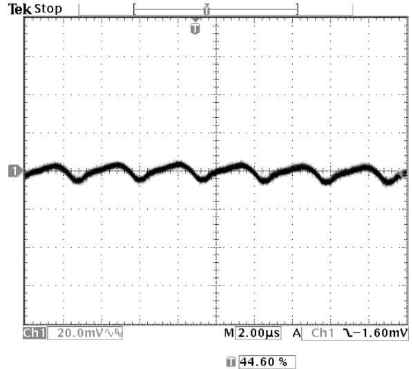
Fig-2.0V-5: Output voltage ripple (20mV/div.) for Vout=2.0V at full rated load current into a resistive load with external capacitance 47uFx2 ceramic + 1uF ceramic at Vin=12V. Time scale: 2 us/div
