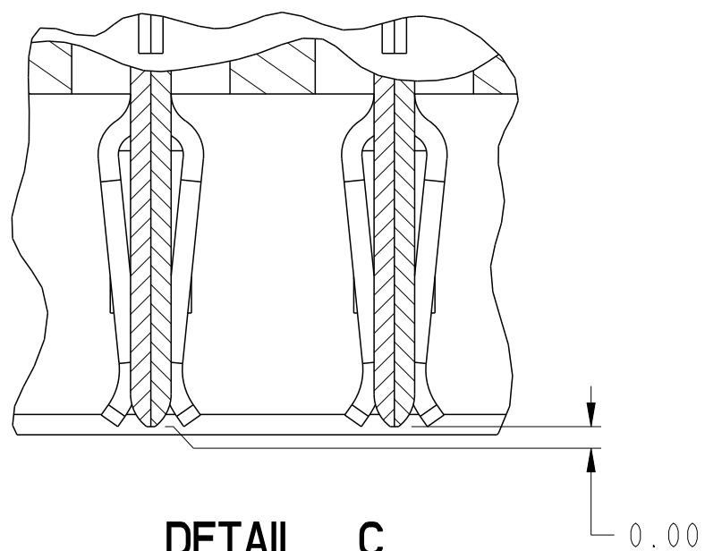
DETAIL C SCALE 6:1
