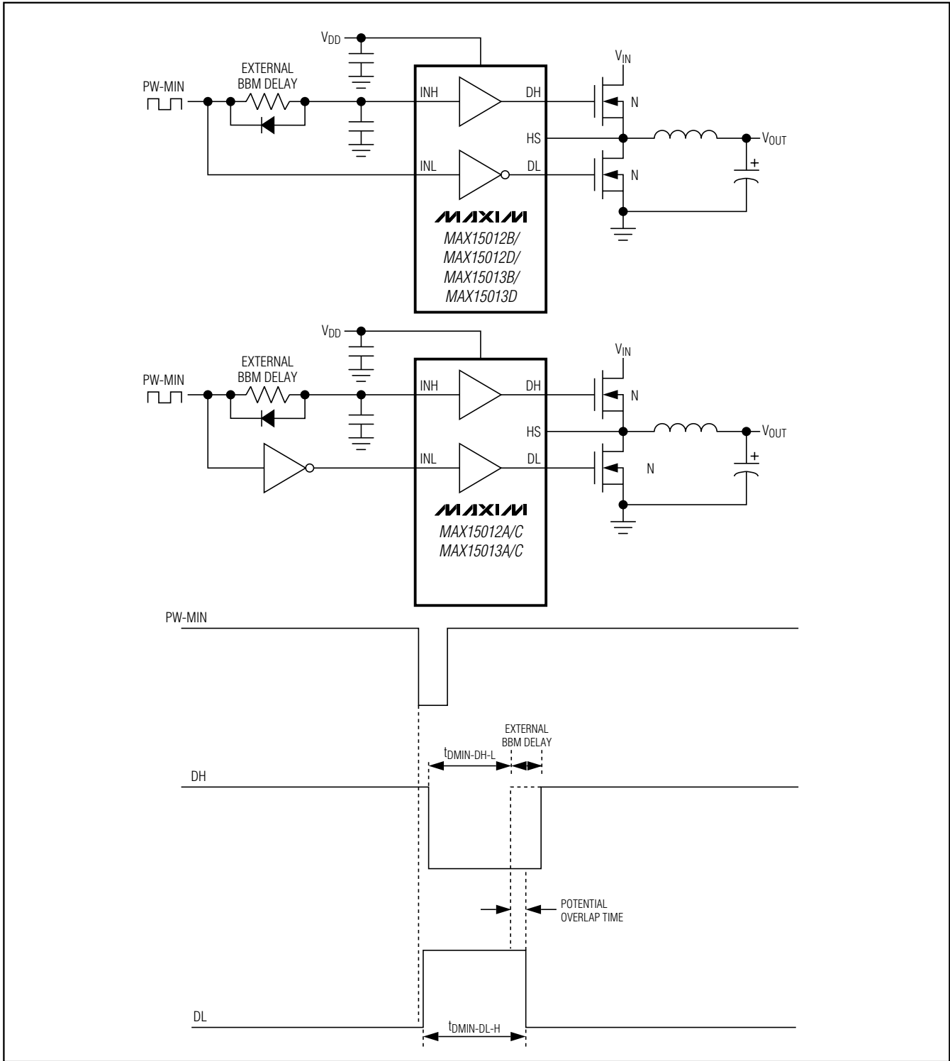
Figure 3. Minimum Pulse-Width Behavior for High Duty-Cycle Input (Off-Time <math>PW_{min}</math>)
