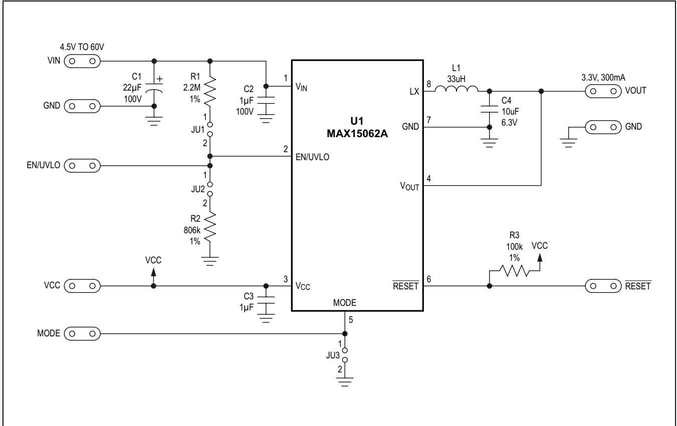
Figure 1. MAX15062A EV Kit Schematic
