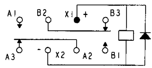
TERMINAL VIEW
