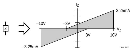
Figure 7. V.11 Interface Using the LTC1344A
