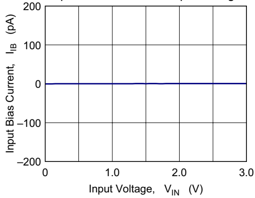
Figure 3-11 HA1631D03 Input Bias Current vs. Input Voltage
