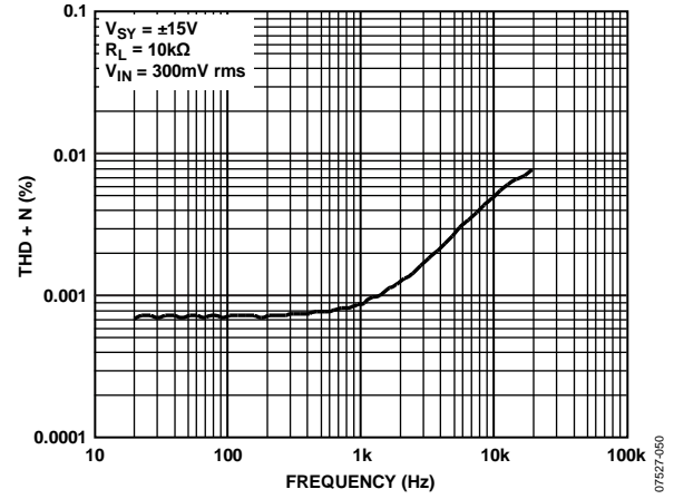
Figure 53. THD + Noise vs. Frequency
