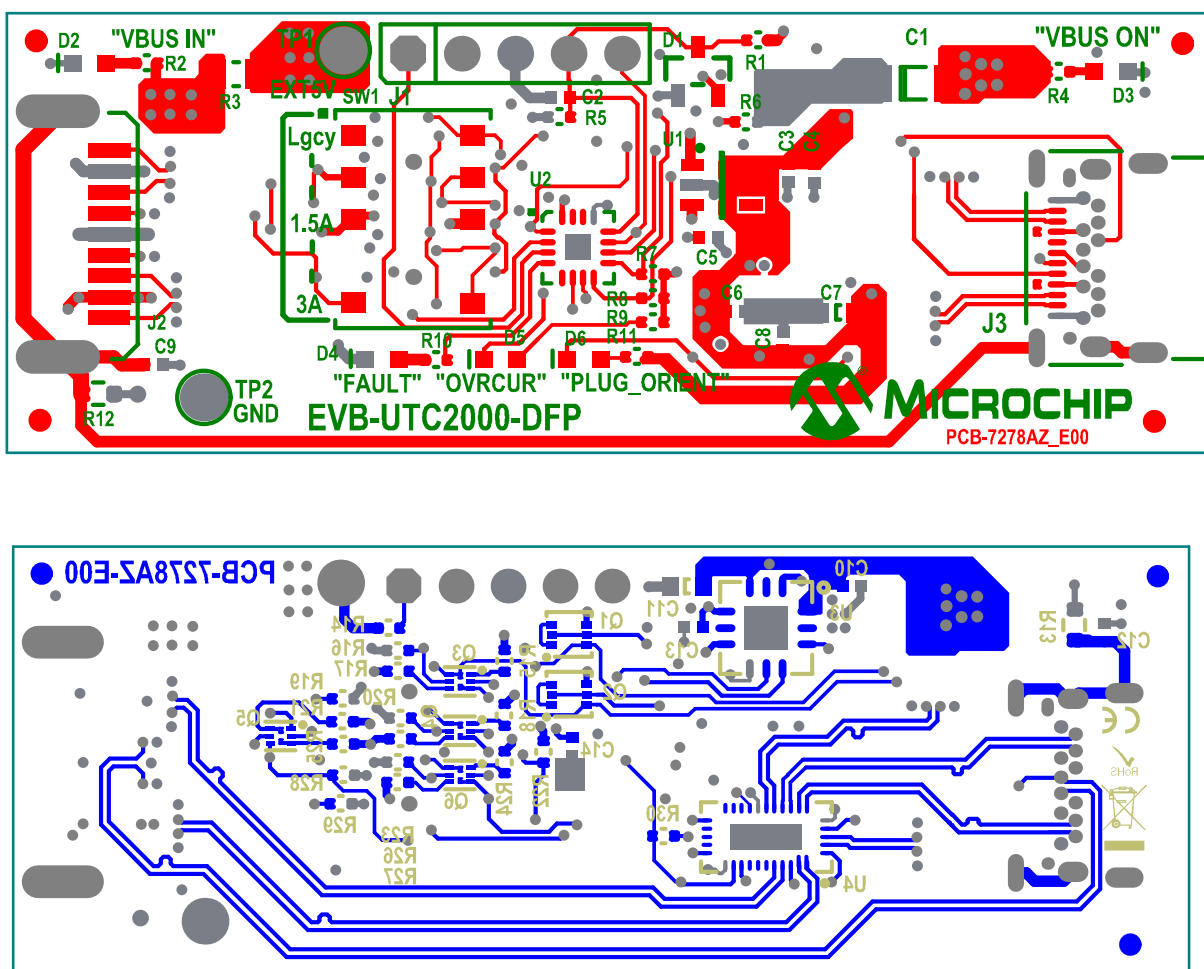
FIGURE C-1: EVB-UTC2000-DFP TOP AND BOTTOM SILK SCREEN IMAGES
