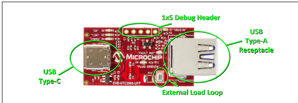
FIGURE 3-7: EVB-UTC2000-UFP LED INDICATOR LOCATIONS
